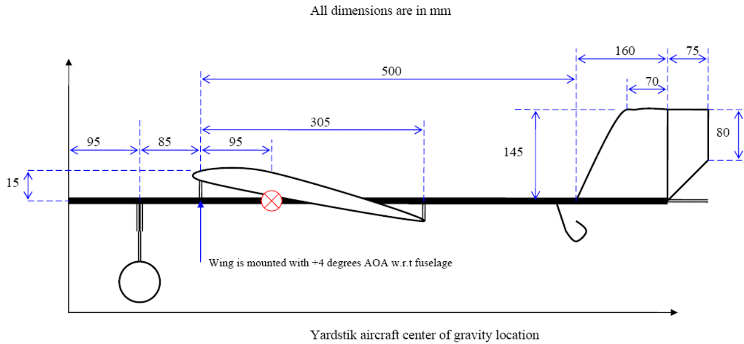
Figure 1 Side view of Yardstik
