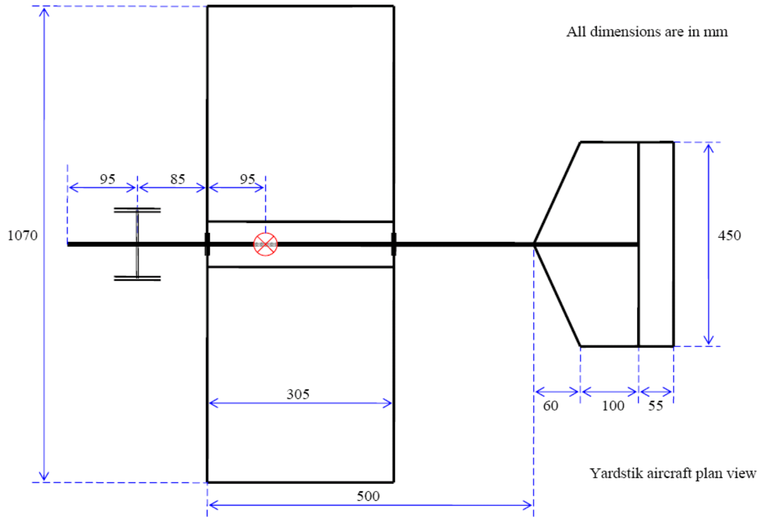
Figure 2 Plan View of Yardstik
